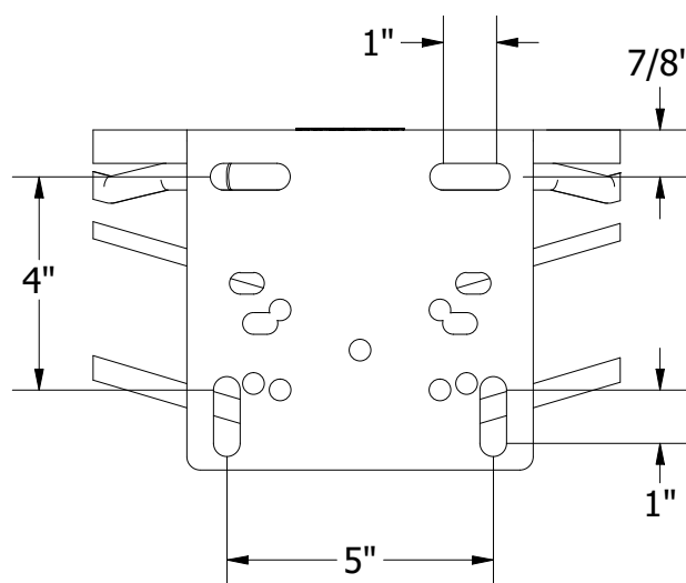
BACK
