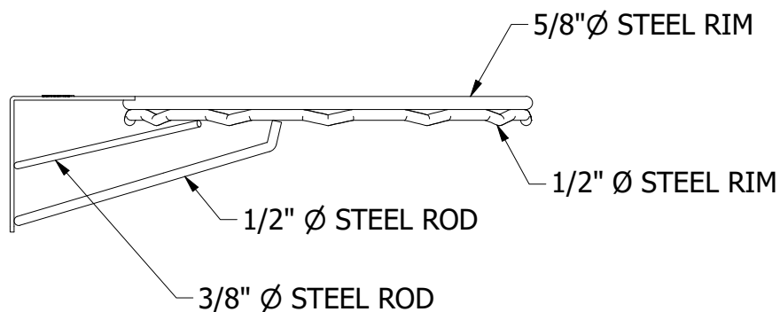
SIDE
